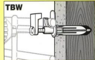
TBW Wire Shelf Anchor with locking retainer clip
